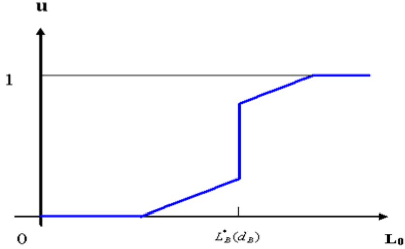
Figure 5(1): Panic effect
