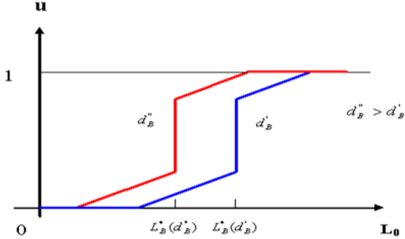
Figure 5(2): Amplifying effect
